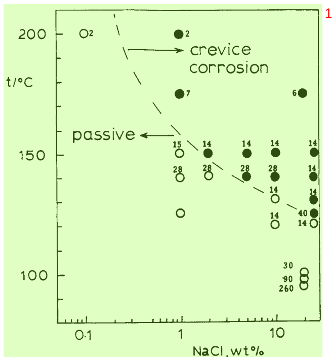
FIGURE 6 — Effect of temperature and chloride concentration on the crevice corrosion of Alloy C-276. The number beside each data point is the exposure time in days; (●) crevice corrosion with obvious metal loss, (○) no corrosion, and (---) tentative crevice temperature envelope.
