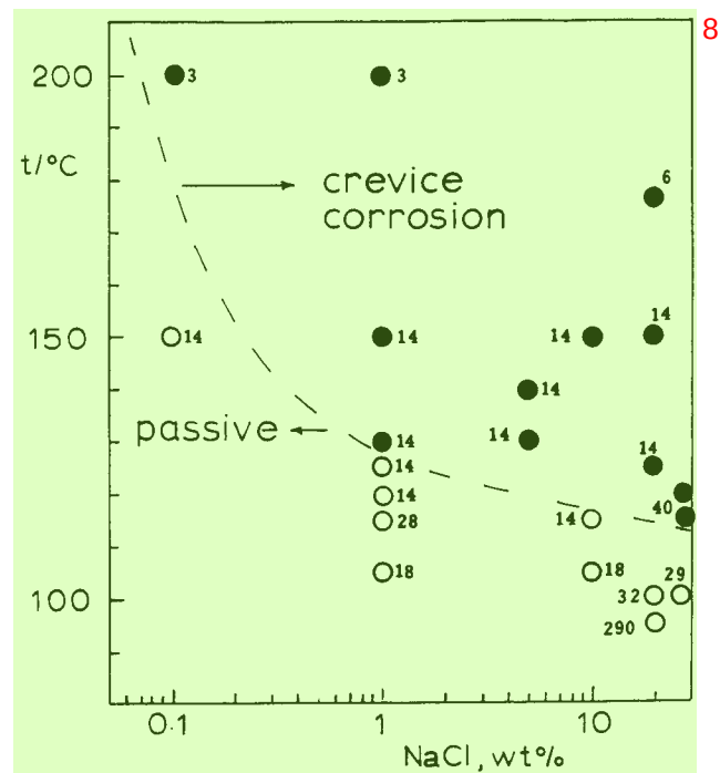
FIGURE 7 — Effect of temperature and chloride concentration on the crevice corrosion of Alloy 625; the number beside each data point is the exposure time in days; (●) crevice corrosion with obvious metal loss, (○) no corrosion, and (---) tentative crevice temperature envelope.
